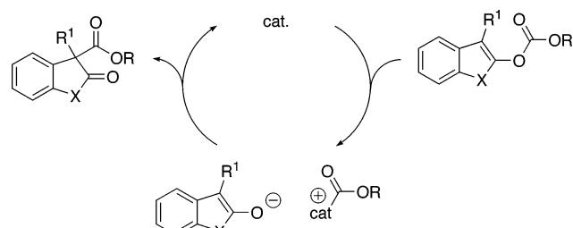
FIGURE 6. Proposed pathway for nucleophile-catalyzed rearrangements of O -acylated enolates.
